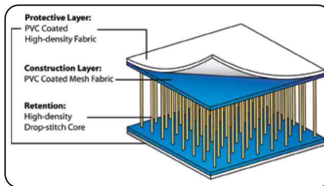
Drop-stitch Construction
